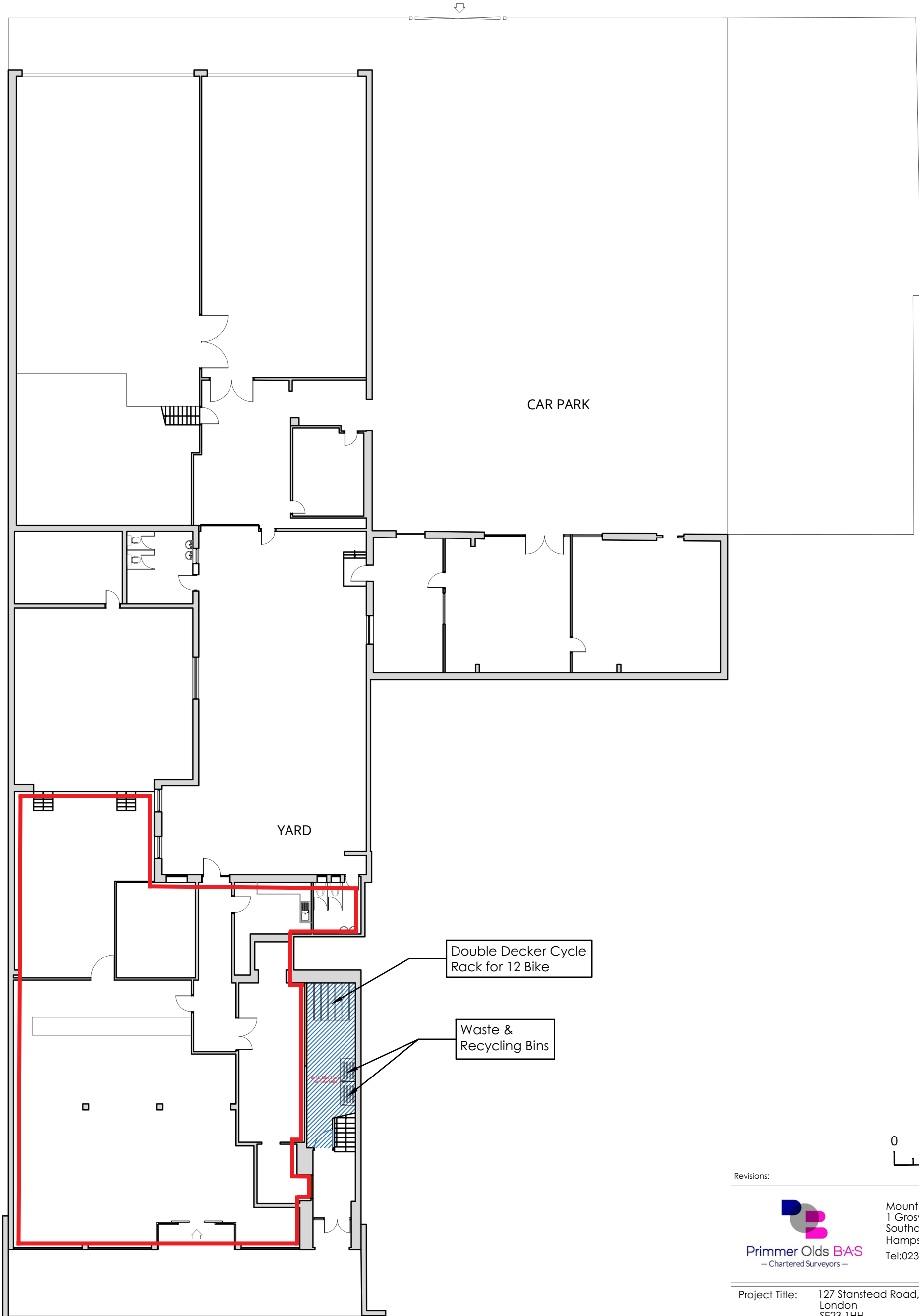
① Proposed Ground Floor Plan Scale 1:200
